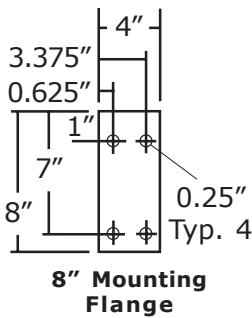
YZ101-W or B-V Vertical Mount
