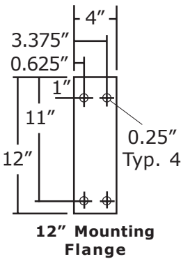
YZ101-W or B-H Horizontal Mount
