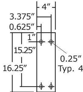
16" Mounting Flange
