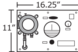
YZ103-W or B-H Horizontal Mount
