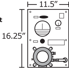
YZ103-W or B-V Vertical Mount
