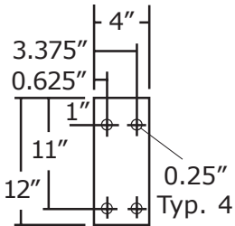
12" Mounting Flange
